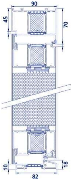
LuxThermo 90 Plus Exclusive U_d=0,7 \text{ W/m}^2\text{K}
