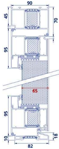
LuxThermo 90 Plus Classic U_d=0,8 \text{ W/m}^2\text{K}
