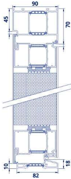
LuxThermo 90 Exclusive U_d=0,8 \text{ W/m}^2\text{K}
