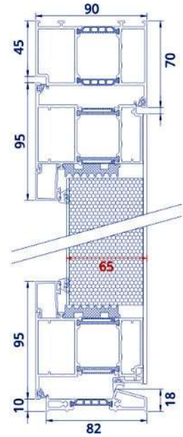
LuxThermo 90 Classic U_d=0,9 \text{ W/m}^2\text{K}
