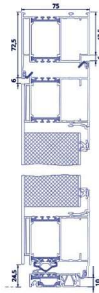
ProThermo 75 Classic U_d=1,1 \text{ W/m}^2\text{K}
